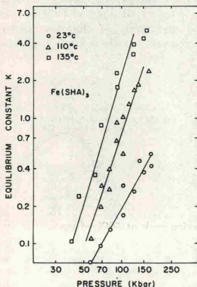
Fig. 3. \text{Ln}K vs. \text{Ln}P for \text{Fe}(\text{SHA})_3 .
