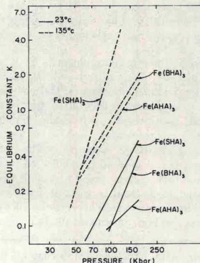
Fig. 4. \text{Ln}K vs. \text{Ln}P for ferric hydroxamates.
